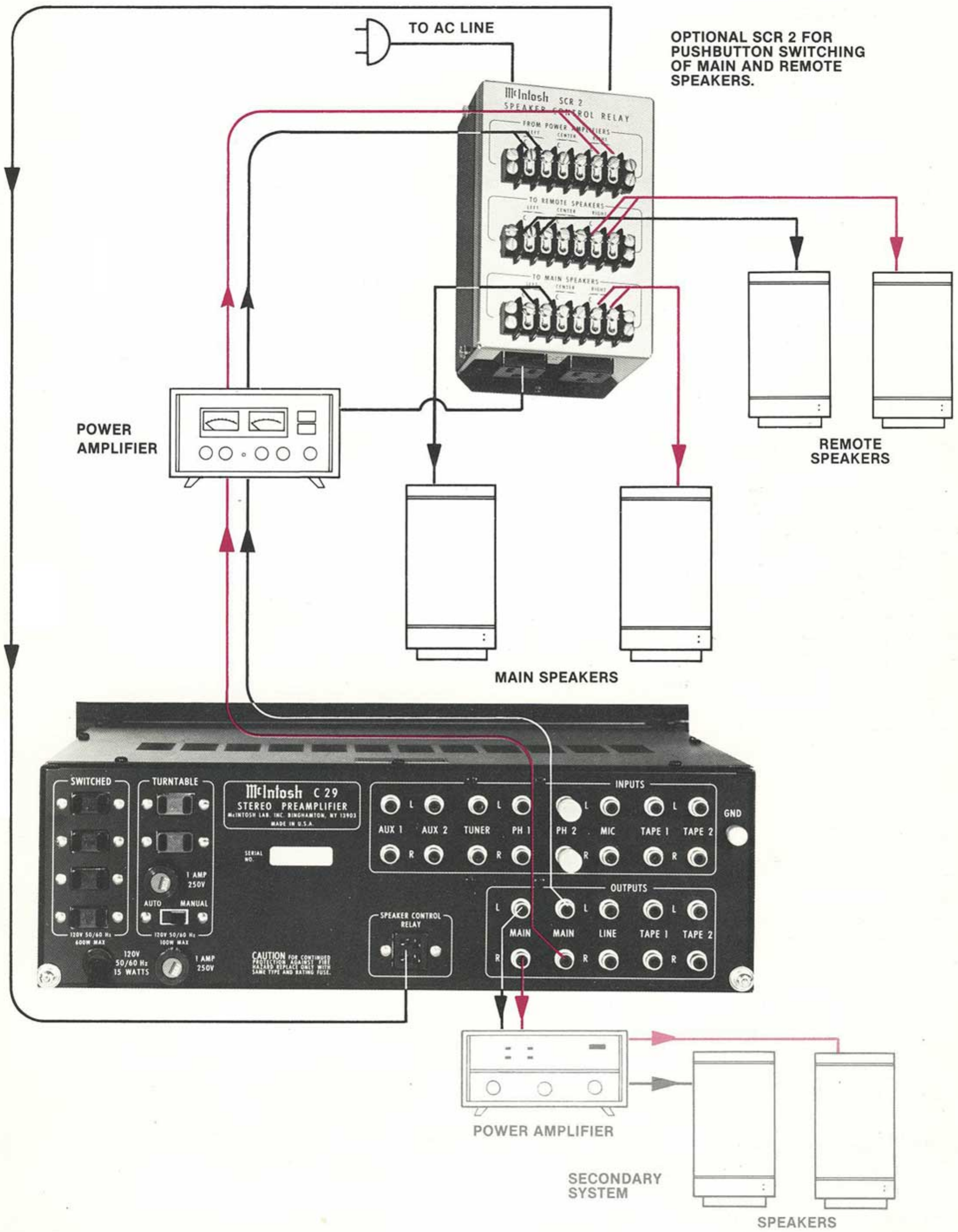
CONNECTIONS FOR POWER AMPLIFIERS AND LOUDSPEAKERS
